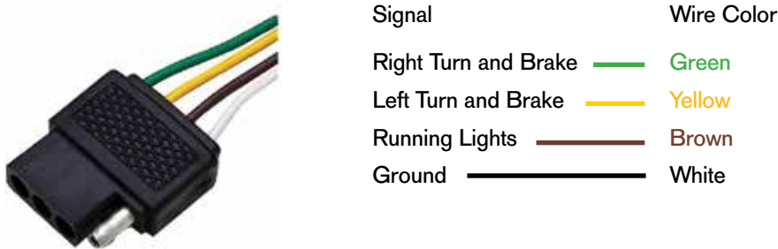
Typical 4-way trailer connection
